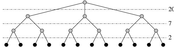
Figure 8: A “tree-leaf” graph of three levels. Processors are drawn in black and routers in grey. The description of this architecture is “ tleaf 3 3 20 2 7 2 2”, since it has 3 levels, the first level has 3 sons and a traversal cost of 20, the second level has 2 sons and a traversal cost of 7, and the third level has also 2 sons and a traversal cost of 2.
