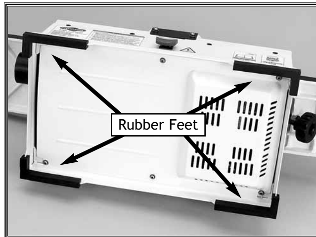
Figure 8. Attached rubber feet.
