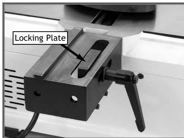
Figure 10. Secured locking plate.
