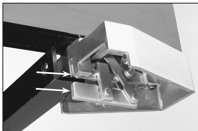
Figure 8. Jaw position.
