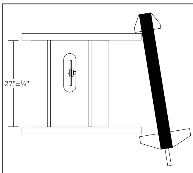
Figure 7. Fence installation.
