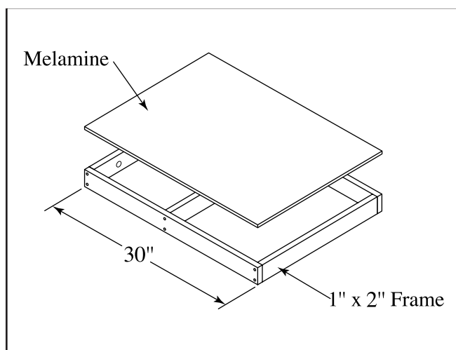
Figure 5. Extension table.
