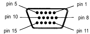
VGA Port Connector Pin Assignments
