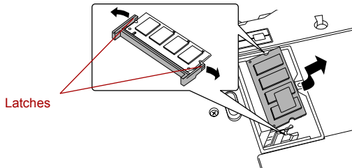
Removing the memory module
