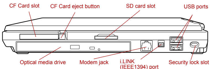
The right side of the computer
