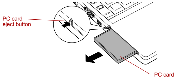
Removing the PC card
