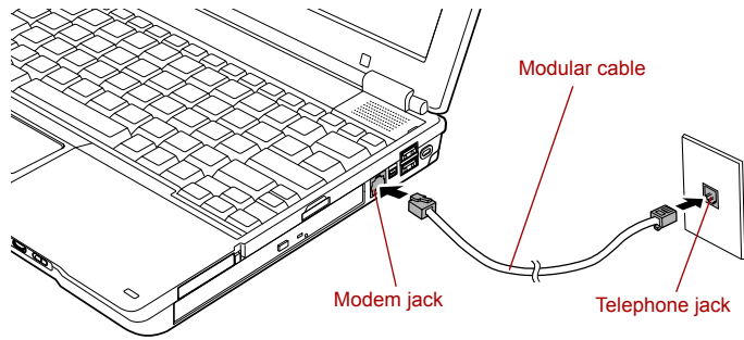
Connecting the internal modem
