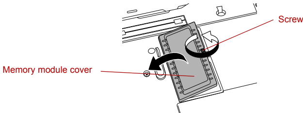
Removing the memory module cover
