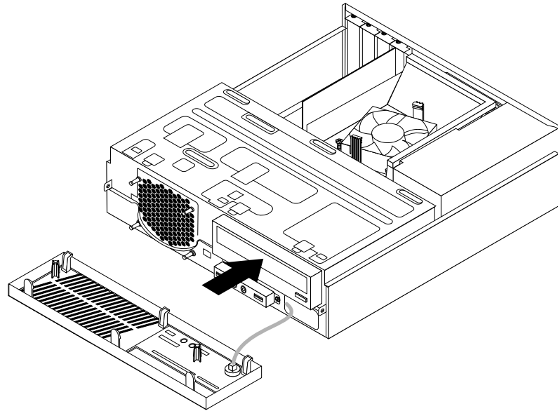
Figure 28. Installing a new optical drive
