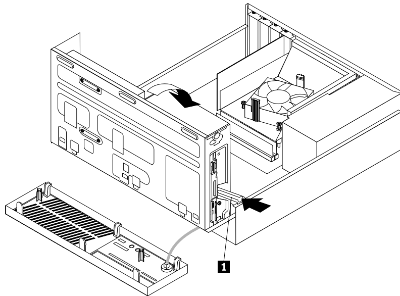
Figure 26. Lowering the drive bay assembly
