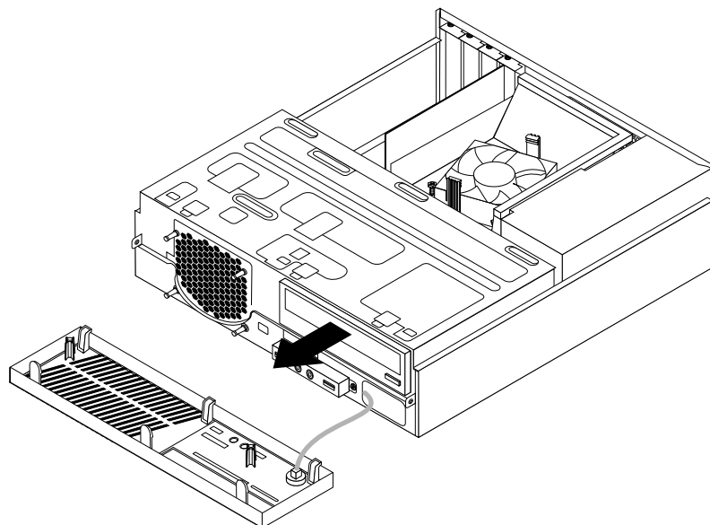
Figure 27. Removing the optical drive
