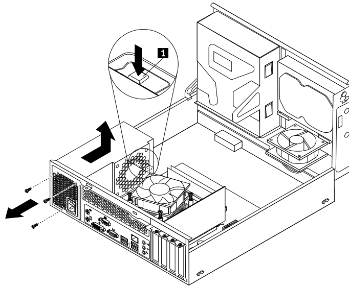
Figure 35. Removing the power supply assembly
