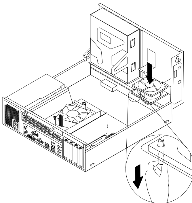
Figure 43. Installing the system fan assembly
