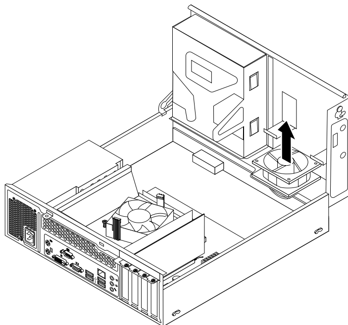
Figure 42. Removing the system fan assembly
