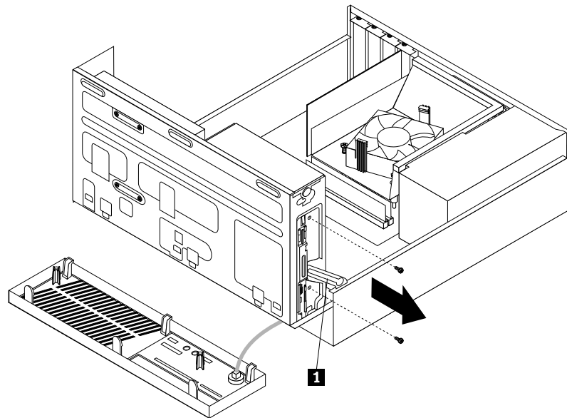
Figure 25. Removing the optical drive screws
