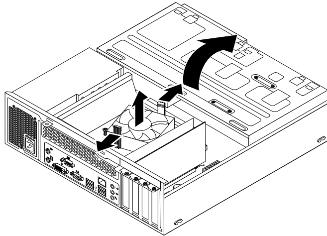
Figure 31. Removing the heat sink fan duct
