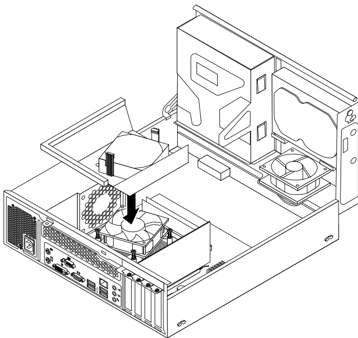
Figure 37. Installing the heat sink fan duct
