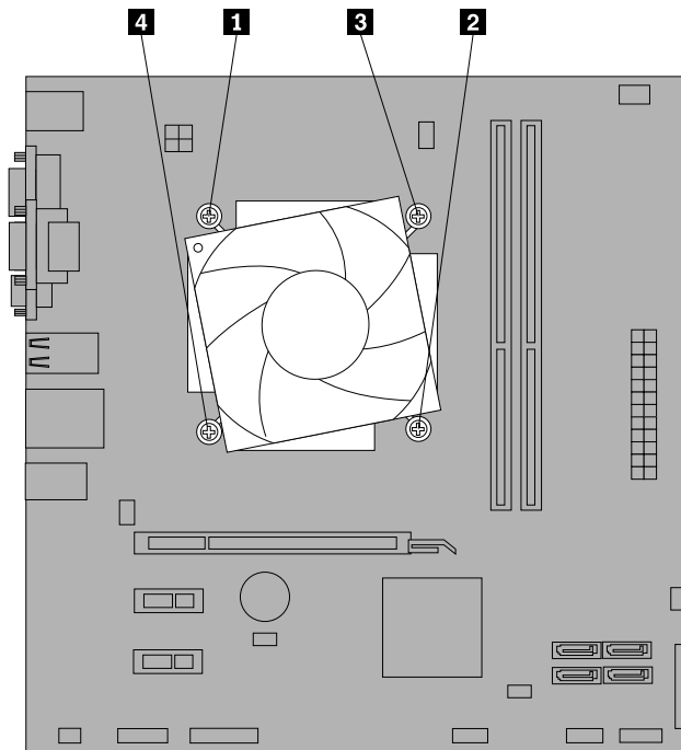
Figure 32. Removing the heat sink and fan assembly
