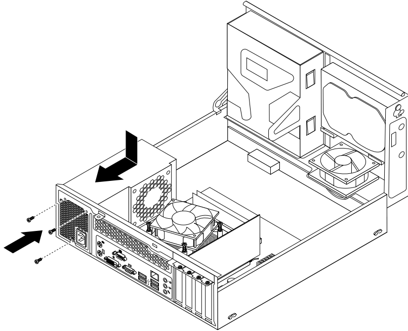
Figure 36. Installing the power supply assembly
