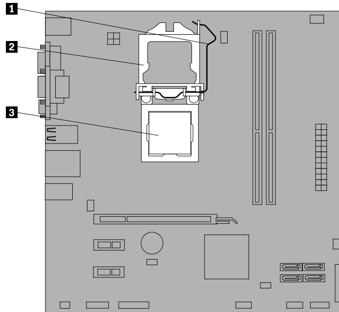
Figure 38. Accessing the microprocessor
