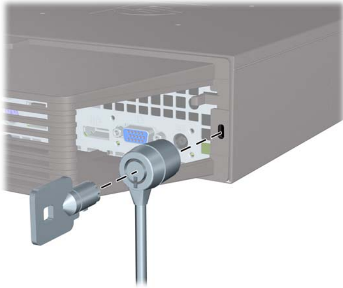
Figure C-2 Installing a Cable with a Port Cover Installed
