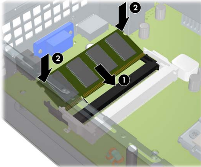
Figure 2-10 Installing a SODIMM
