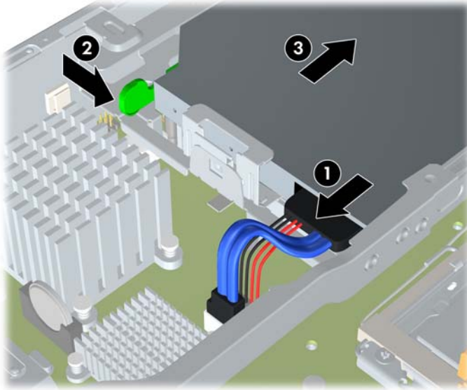
Figure 2-11 Removing the Optical Drive
