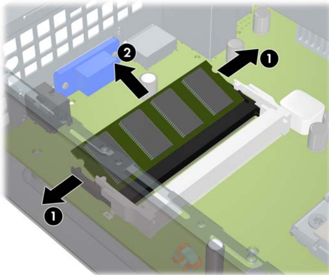
Figure 2-9 Removing a SODIMM
