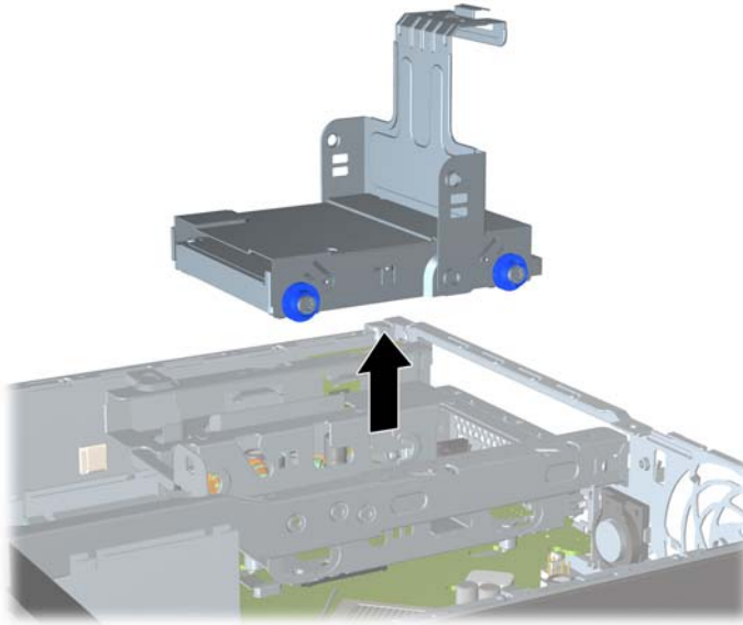
Figure 2-15 Removing the Hard Drive Carrier
