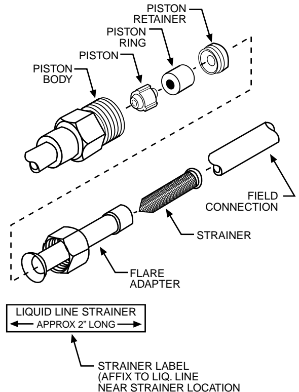
Fig. 4—Check-Flo-Rater® Components (550A, 552A Only)
