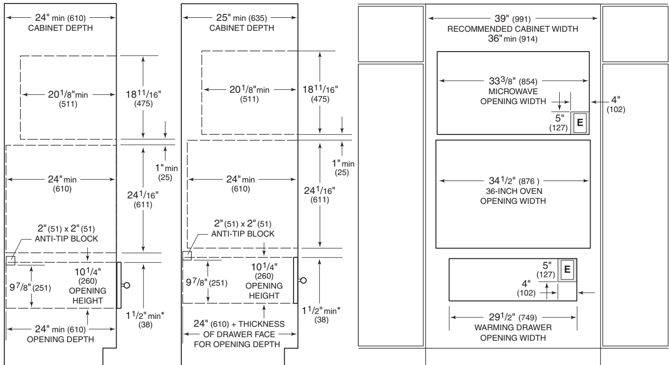
OVERLAY APPLICATION
