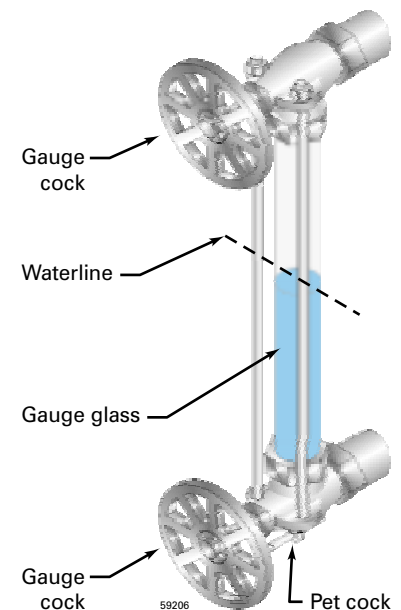
Figure 9 Gauge glass
