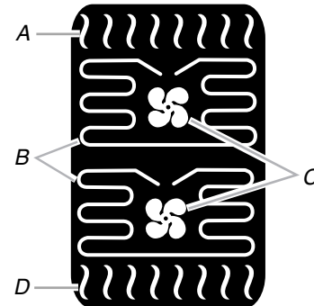
A. Broil element B. Convection elements C. Convection fans D. Bake element
