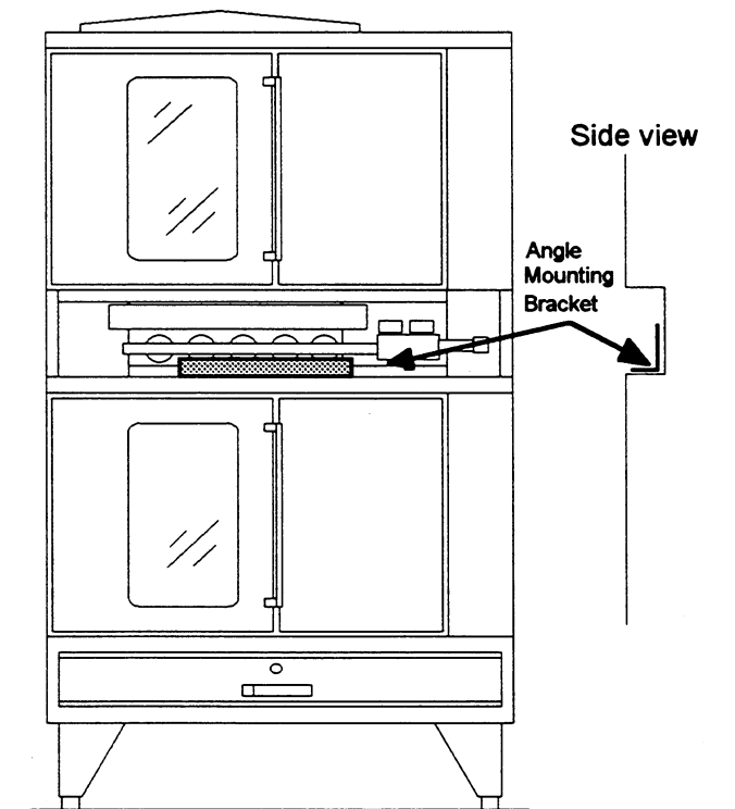
Front view with top combustion cover removed.
