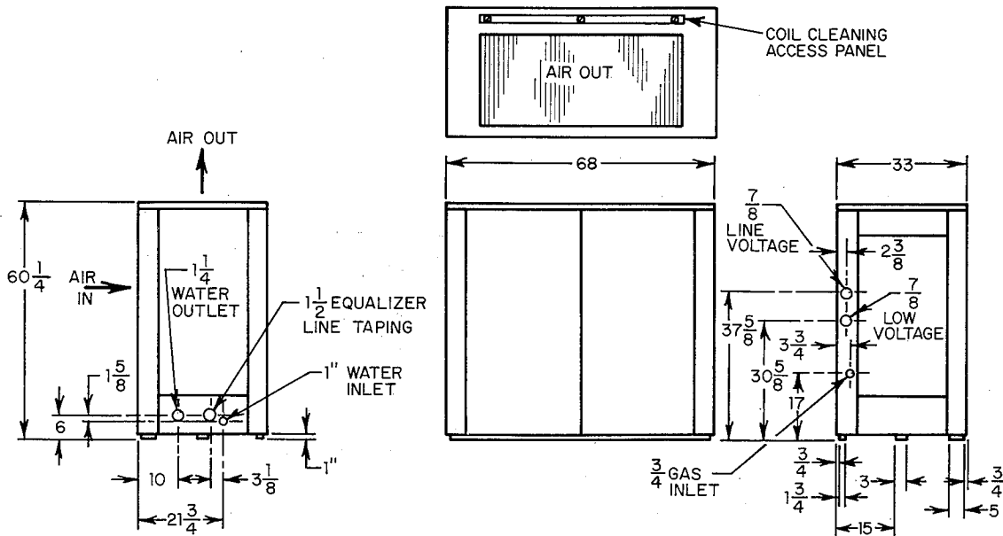
Figure 2 - Dimensional Drawing
