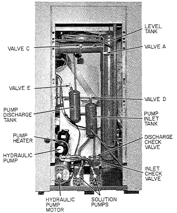
Figure 5 - Unit Right-Side View With Access Panel Removed
