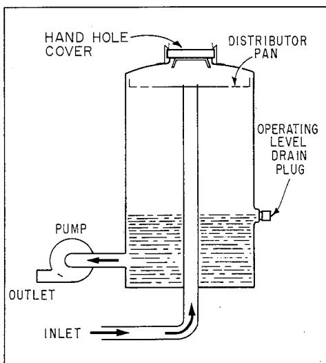
Figure 8 - Chiller Tank
