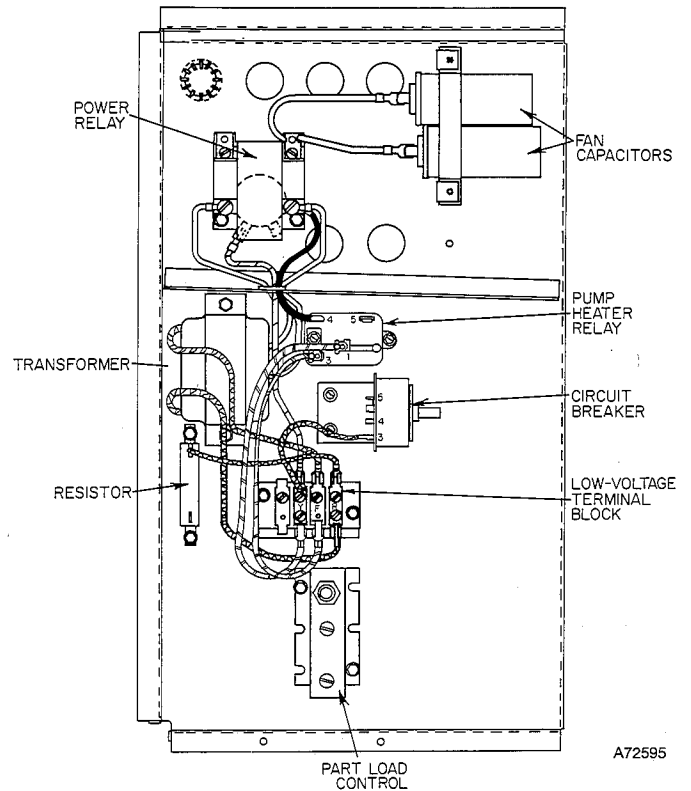
Figure 6 - Control Box Components
