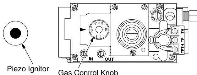
Figure 47 - Control Valve
