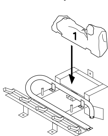
Figure 42 - Installing Log No. 1
