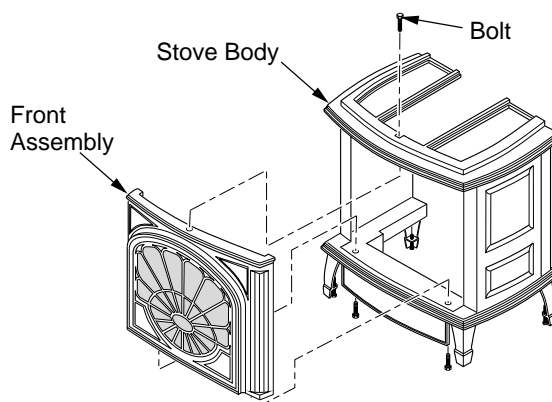
Figure 13 - Removing Front Assembly (Amity™ Model Shown)
