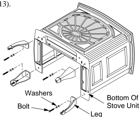
Figure 10 - Attaching Stove Legs (Amity™ Model Shown)
