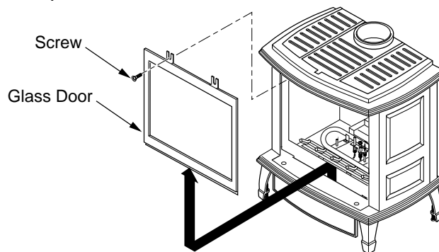
Figure 41 - Removing Glass Door from Burner System
