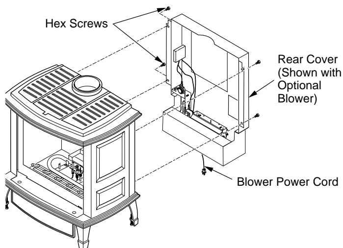
Figure 19 - Installing Rear Cover (Shown with Optional Blower Accessory)
