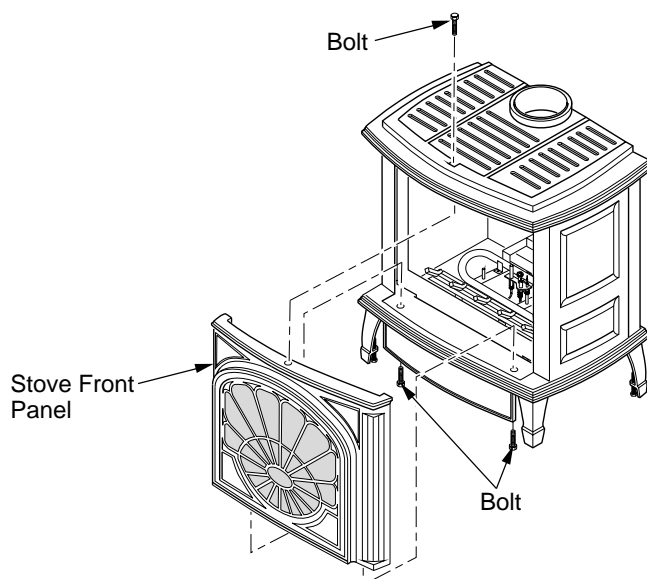
Figure 40 - Removing Front Panel from Stove (Amity™ Model Shown)
