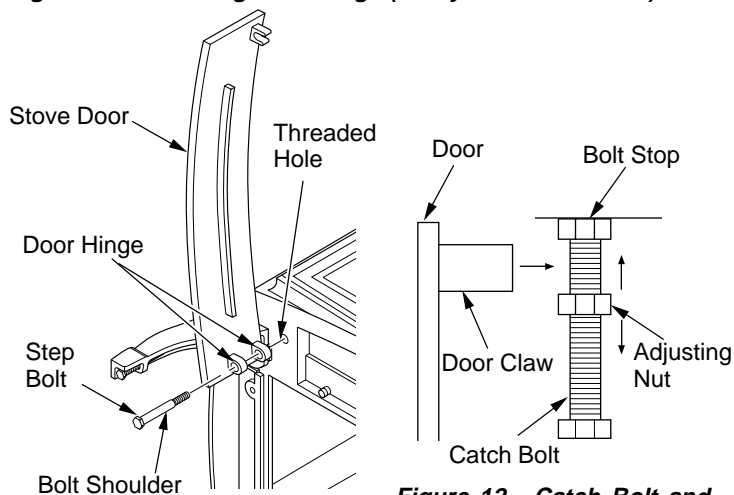
Figure 11 - Attaching Stove Door Figure 12 - Catch Bolt and Door Claw Orientation
