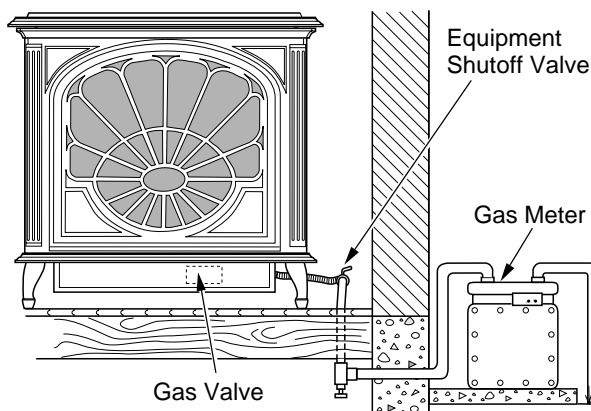
Figure 32 - Checking Gas Joints for Natural Gas Burner System (Amity™ Model Shown)
