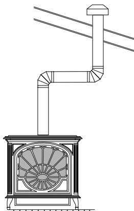
Figure 21 - Vertical Venting Through Ceiling Using Two 90° Elbows (Amity™ Model Shown)
