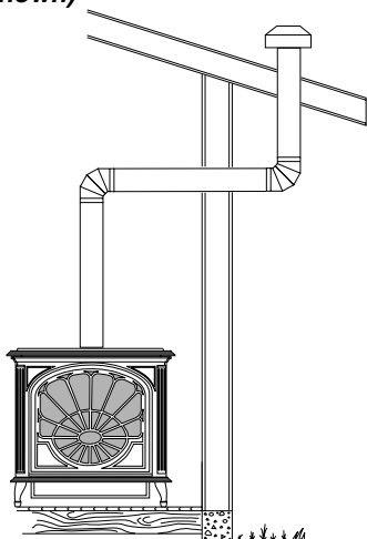
Figure 23 - Venting Through a Side Wall (Amity™ Model Shown)
