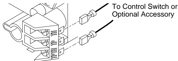
Figure 33 - Control Valve Terminals
