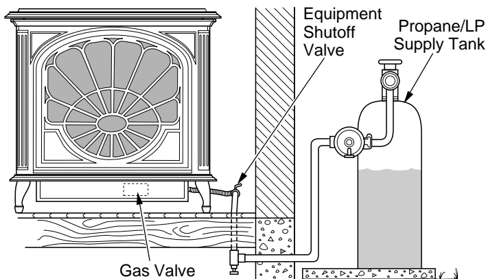
Figure 30 - Checking Gas Joints for Propane/LP Gas Burner System (Amity™ Model Shown)
