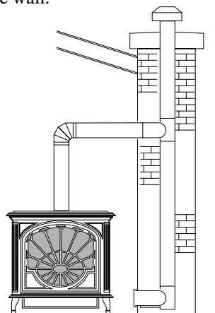
Figure 22 - Vertical Venting Configuration Through Chimney (Amity™ Model Shown)
