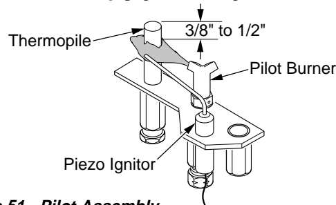
Figure 51 - Pilot Assembly
