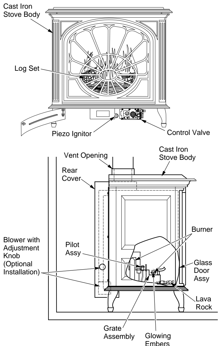
Figure 1 - DESA B-Vent Burner System Shown Installed in Approved DESA Cast Iron Stove Body Models SCIVFC, PSCIVFC, and VH Series Only (Amity™ Model Shown)
