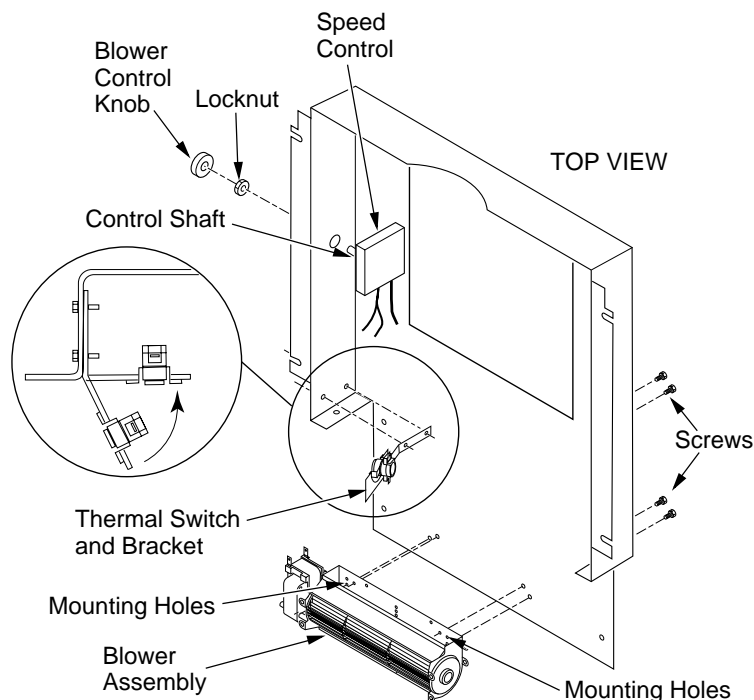
Figure 17 - Blower Assembly, Speed Control, and Thermal Switch Locations
