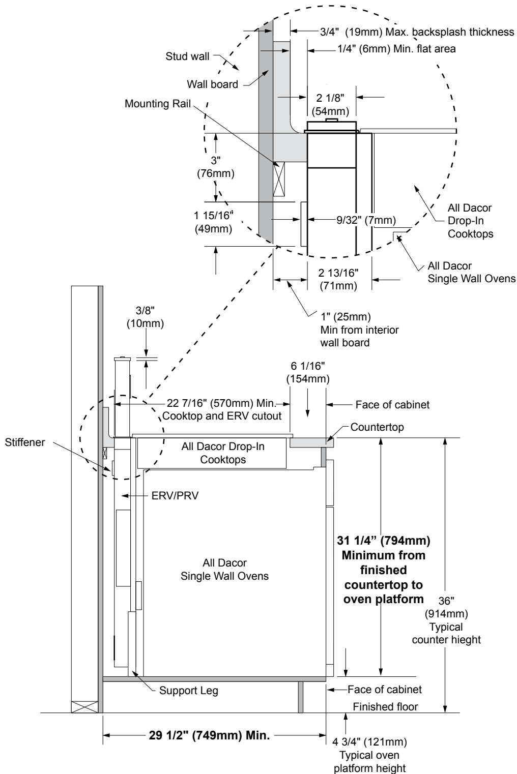
CUTAWAY SIDEVIEW
