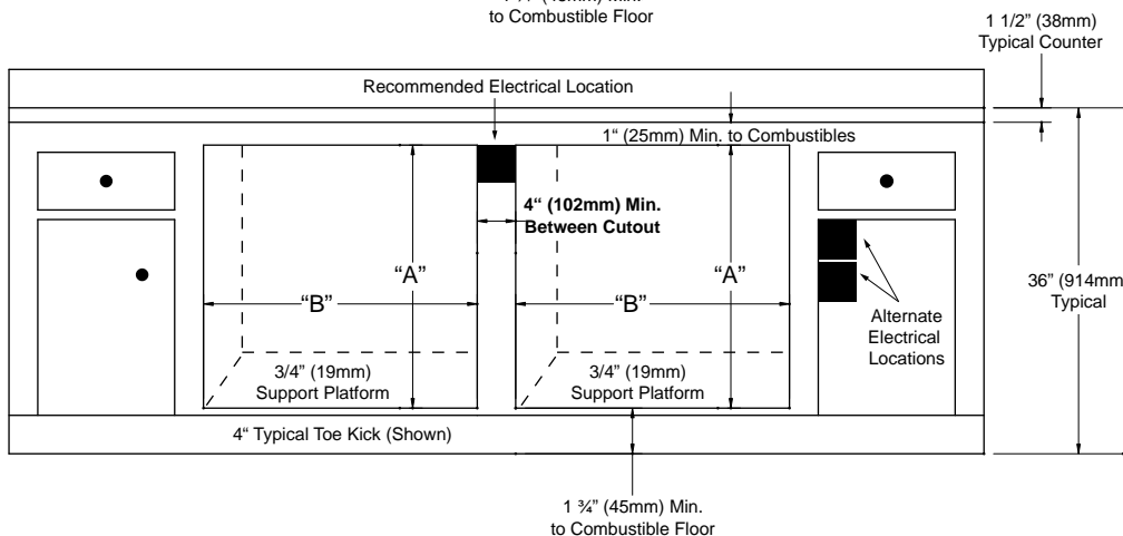
Dual Single Wall Oven Under Counter Cutout
