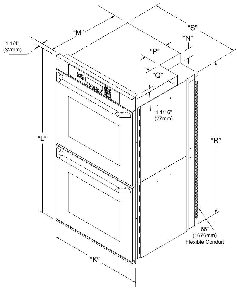
Double Wall Oven Dimension
