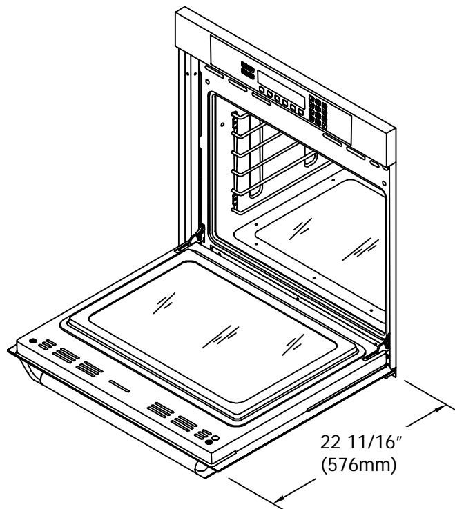
Door Dimension - All Models
