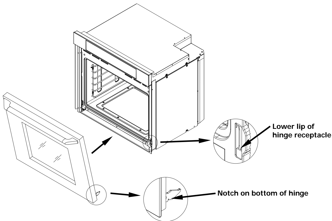
Door Installation
