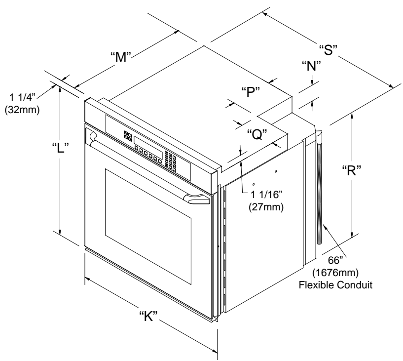
Single Wall Oven Dimension
