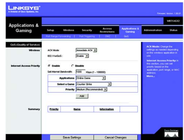
Figure 5-34: QoS - Online Game
