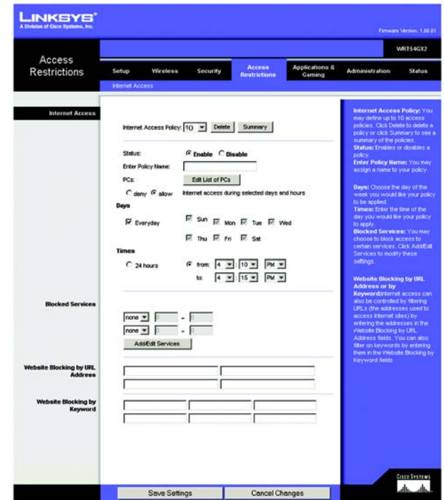
Figure 5-25: Access Restrictions Tab - Internet Access
