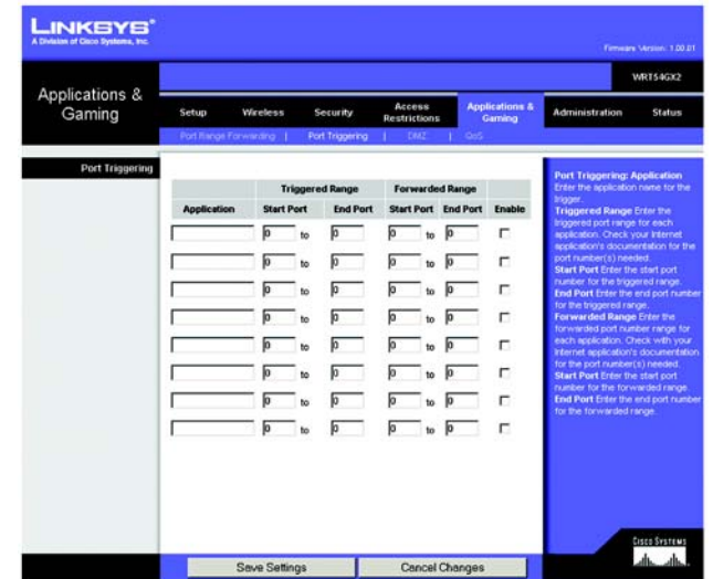
Figure 5-30: Applications and Gaming Tab - Port Triggering
