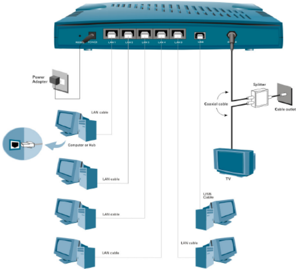
Figure 2-2 Prestige Rear Panel and Connections
