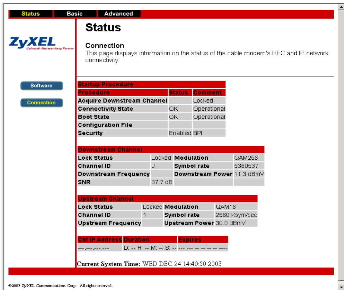
Figure 3-2 Web Management - Status
