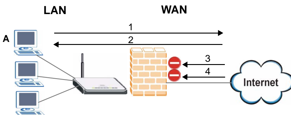
Figure 73 Default Firewall Action
