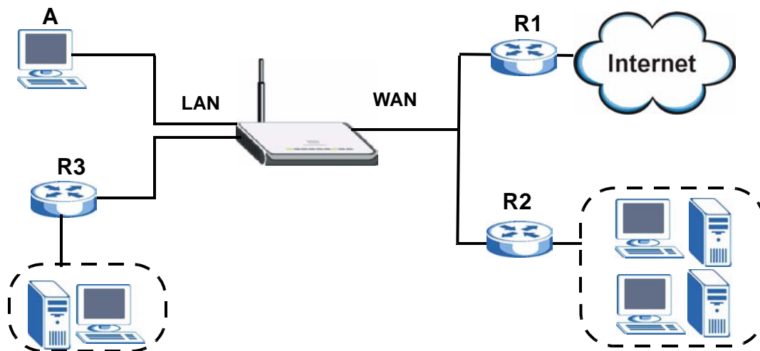
Figure 77 Example of Static Routing Topology
