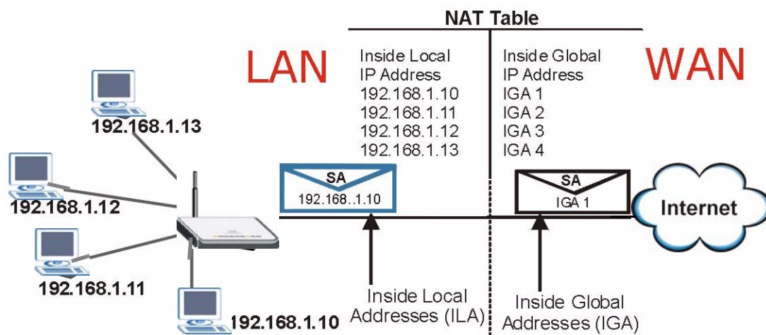
Figure 66 How NAT Works
