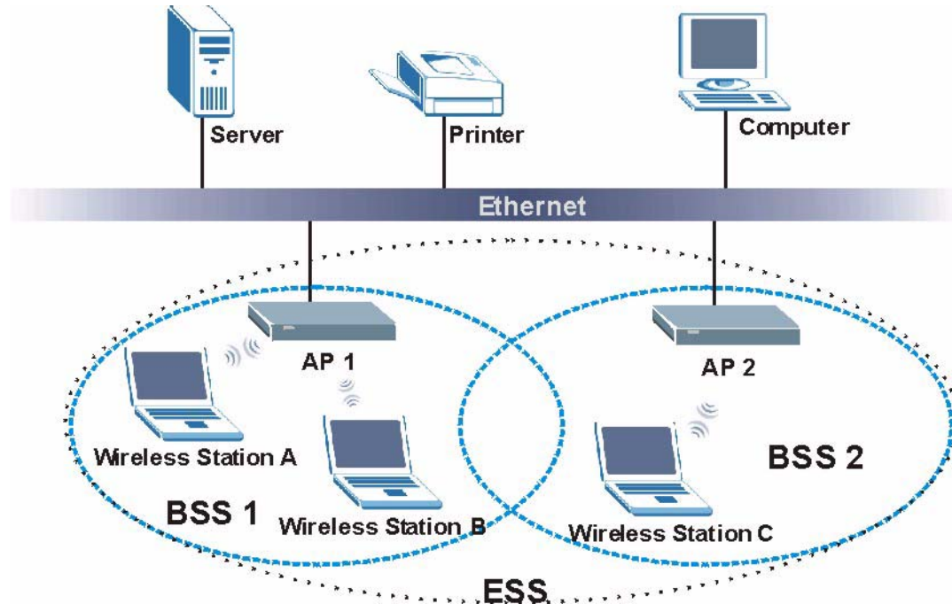
Figure 152 Infrastructure WLAN
