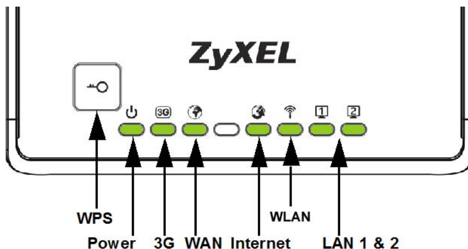
Figure 2 Front Panel
