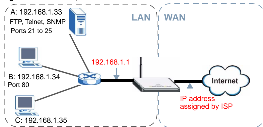
Figure 65 NAT Example
