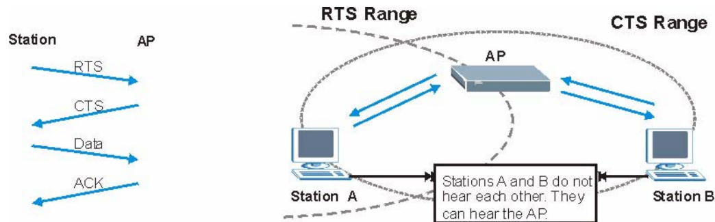
Figure 153 RTS/CTS
