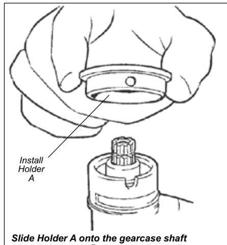
Slide Holder A onto the gearcase shaft
