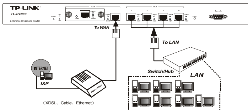
Figure 2-1 Hardware Installation of the TL-R4000 Enterprise Broadband Router
