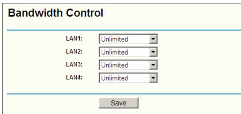
Figure 4-11 Bandwidth Control
