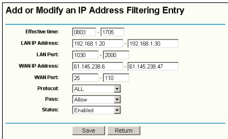
Figure 4-29 Add or Modify an IP Address Filtering Entry
