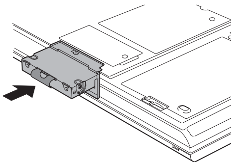
Inserting the new hard disk drive
