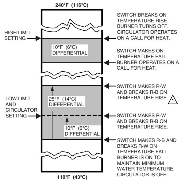
Fig. 7—Relationship of setpoints and differential.
