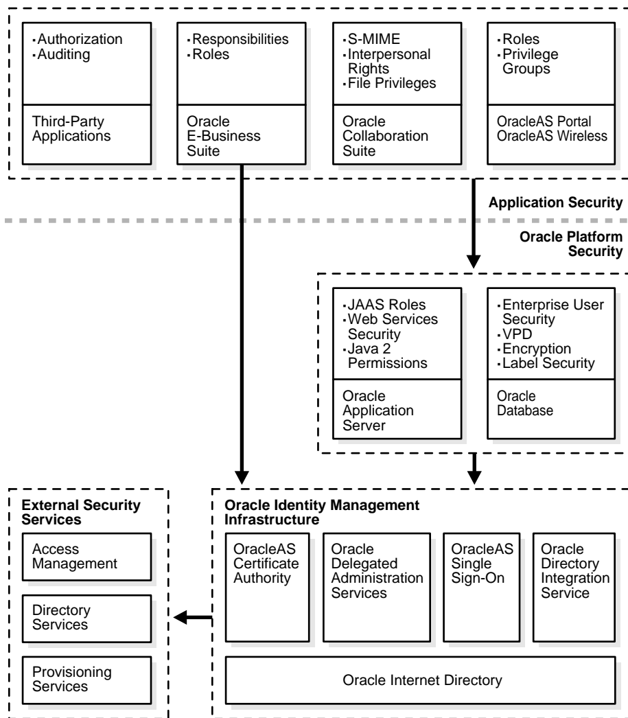
Figure 11–1 Enterprise User Security and the Oracle Security Architecture
