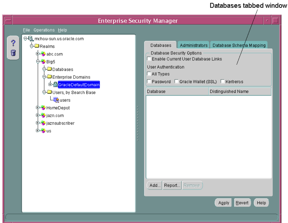
Figure 2–6 Enterprise Security Manager Databases Tabbed Window
