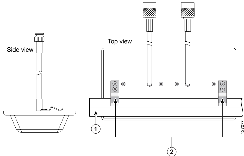
Figure 7 Suspended Ceiling with Flush Mounted Tiles
