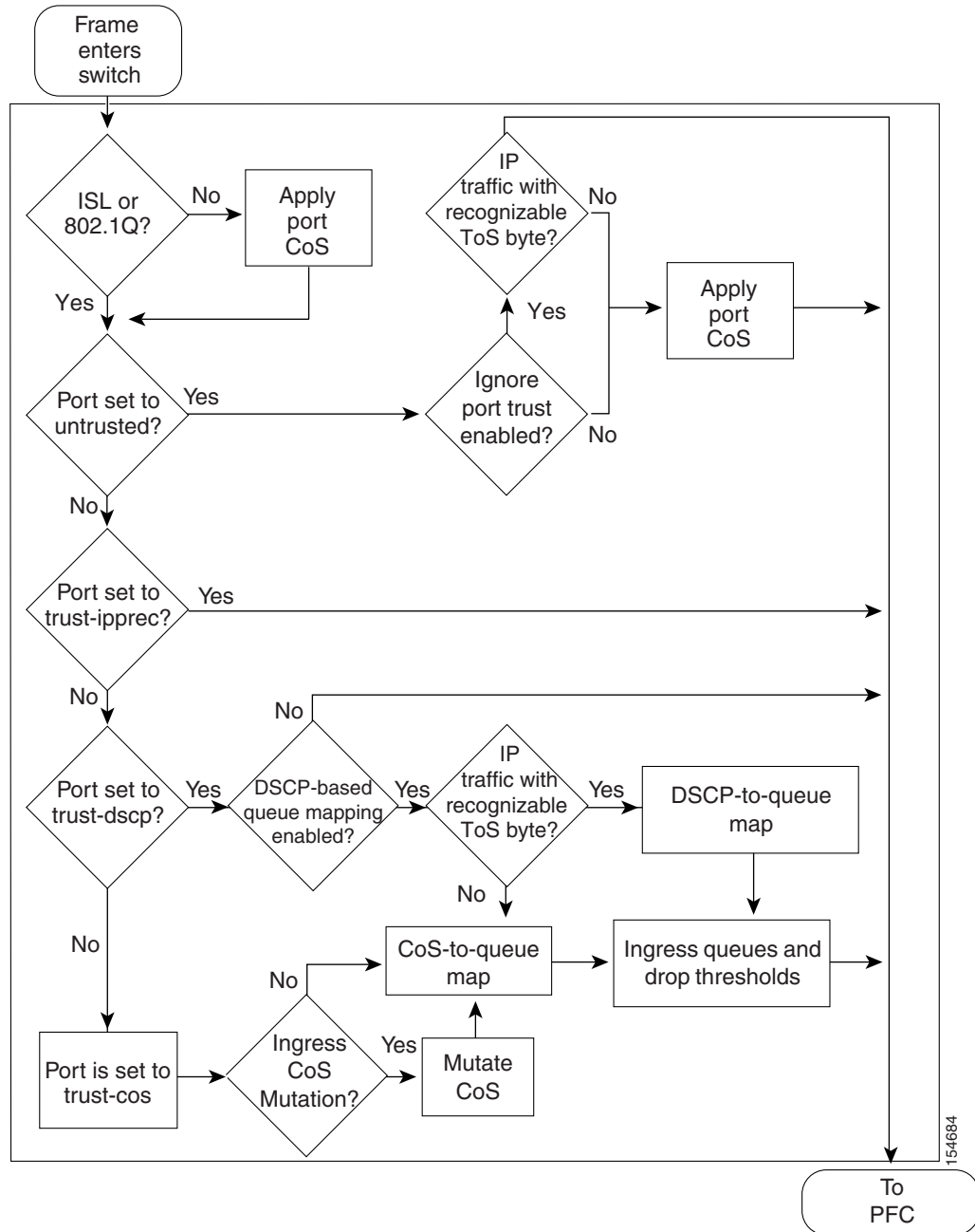
Figure 42-5 Ingress LAN Port PFC QoS Features
