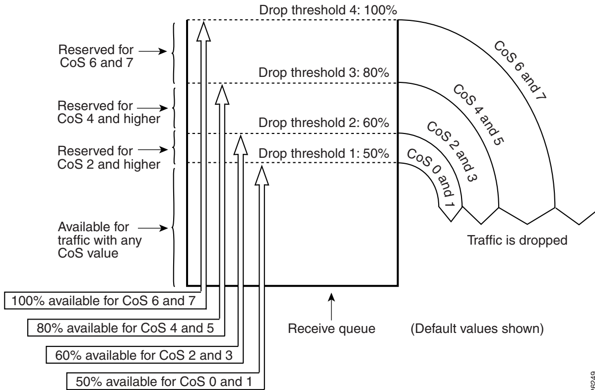
Figure 42-10 Receive Queue Drop Thresholds
