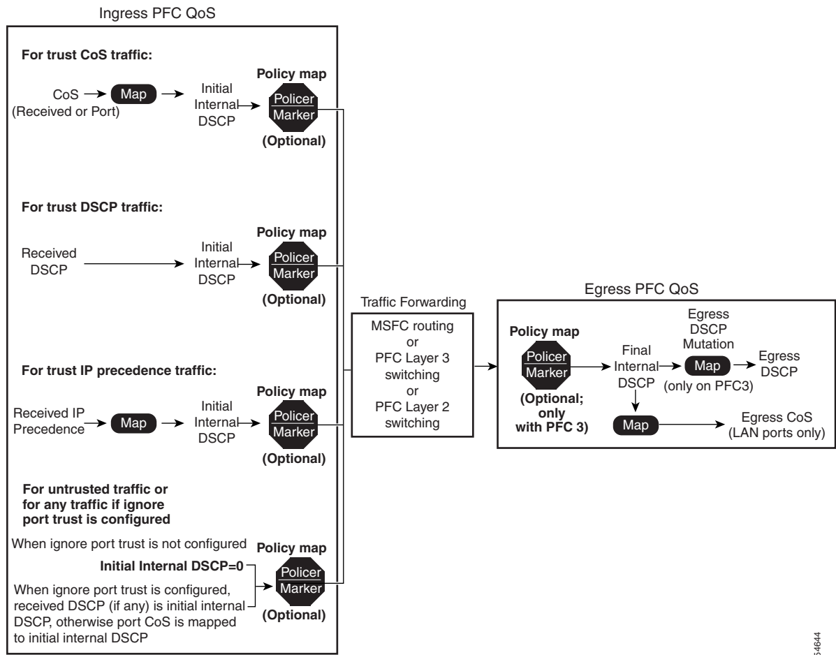
Figure 42-6 QoS Features on the PFC and DFCs
