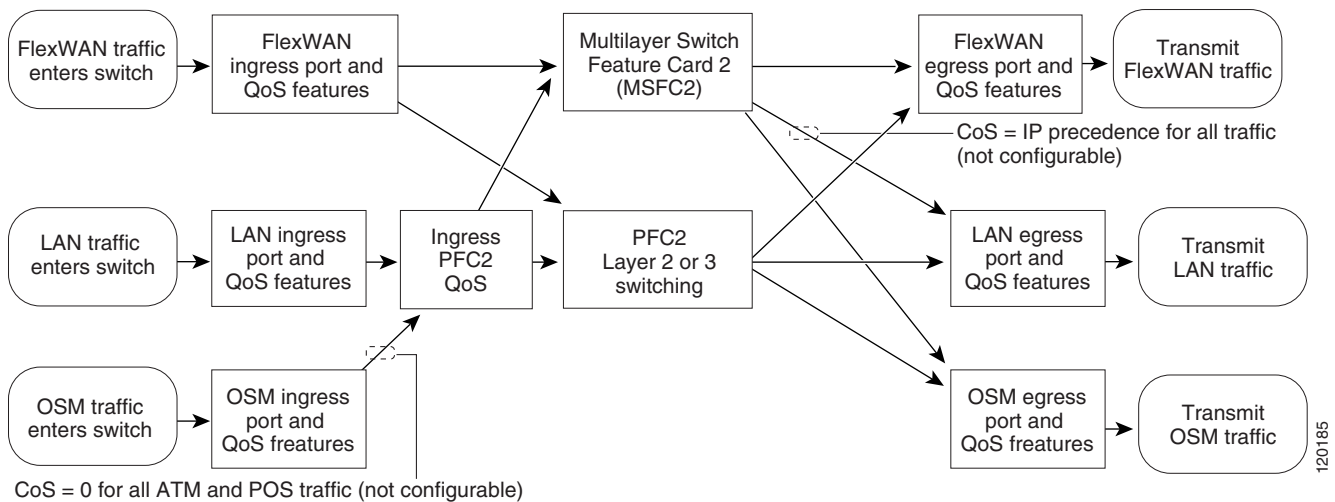
Figure 42-3 Traffic Flow and PFC QoS Features with PFC2
