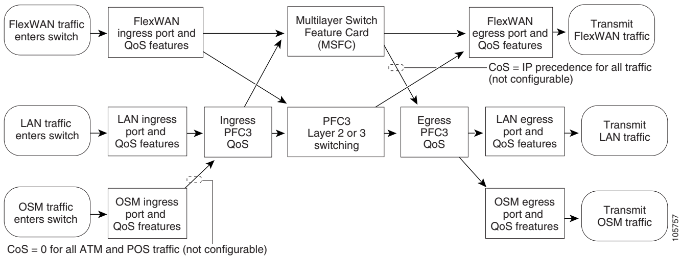
Figure 42-2 Traffic Flow and PFC QoS Features with PFC3
