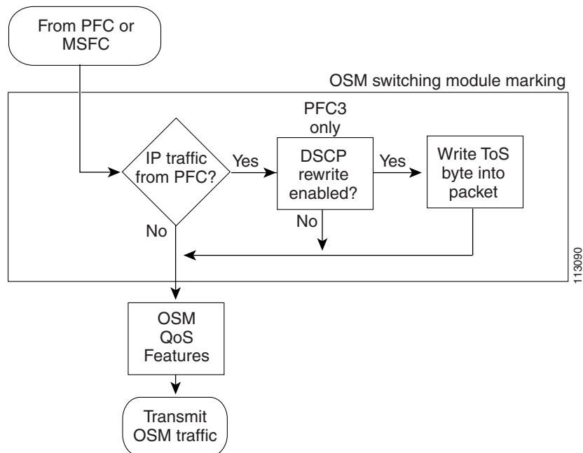
Figure 42-8 Egress OSM Port Marking
