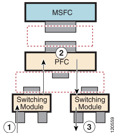
Figure 42-1 PFC QoS Feature Processing Overview
