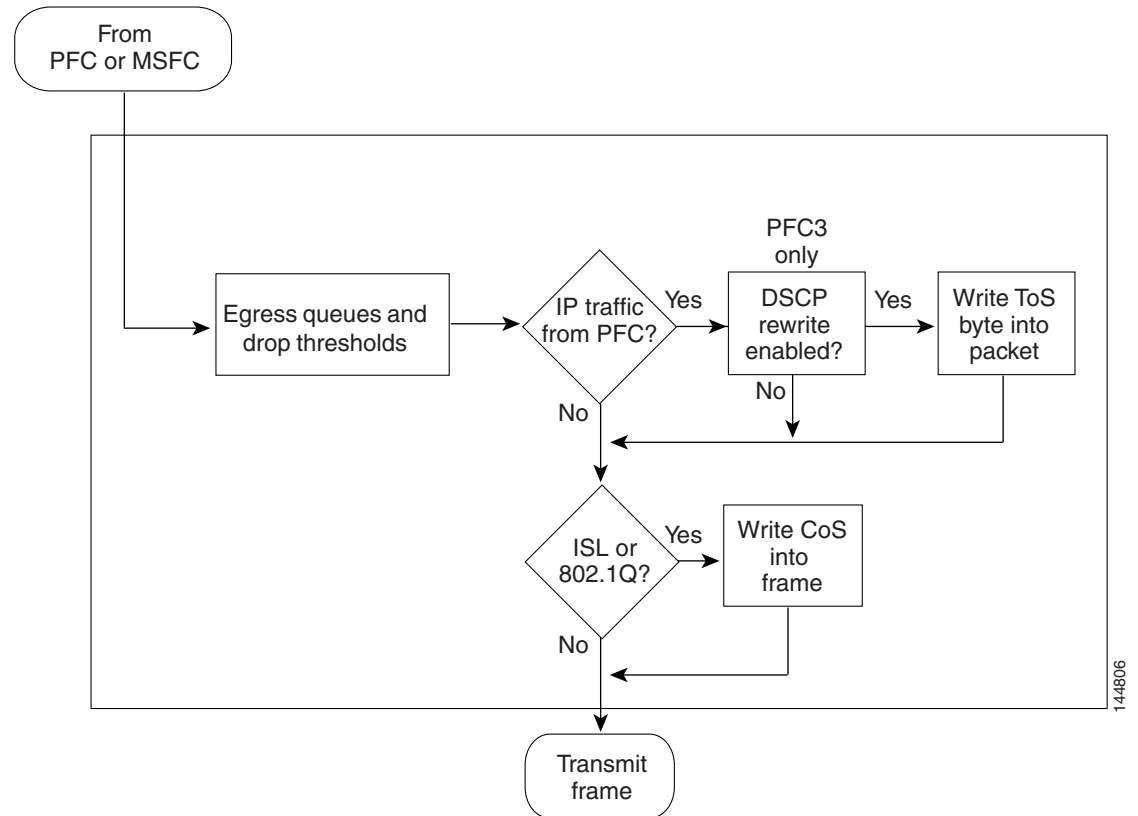
Figure 42-7 Egress LAN Port Scheduling, Congestion Avoidance, and Marking
