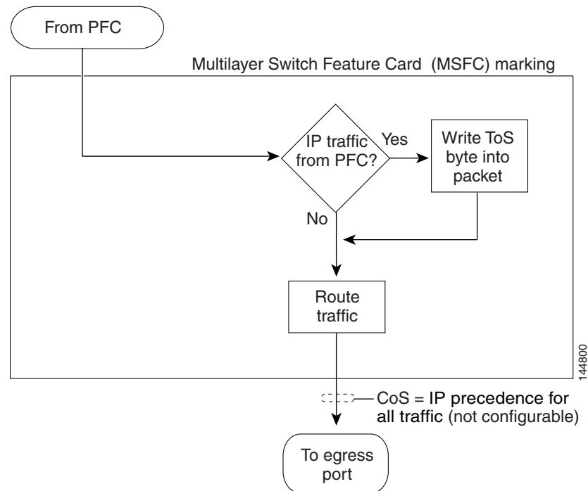
Figure 42-9 Marking with PFC2 or PFC3 and MSFC2, MSFC2A, or MSFC3
