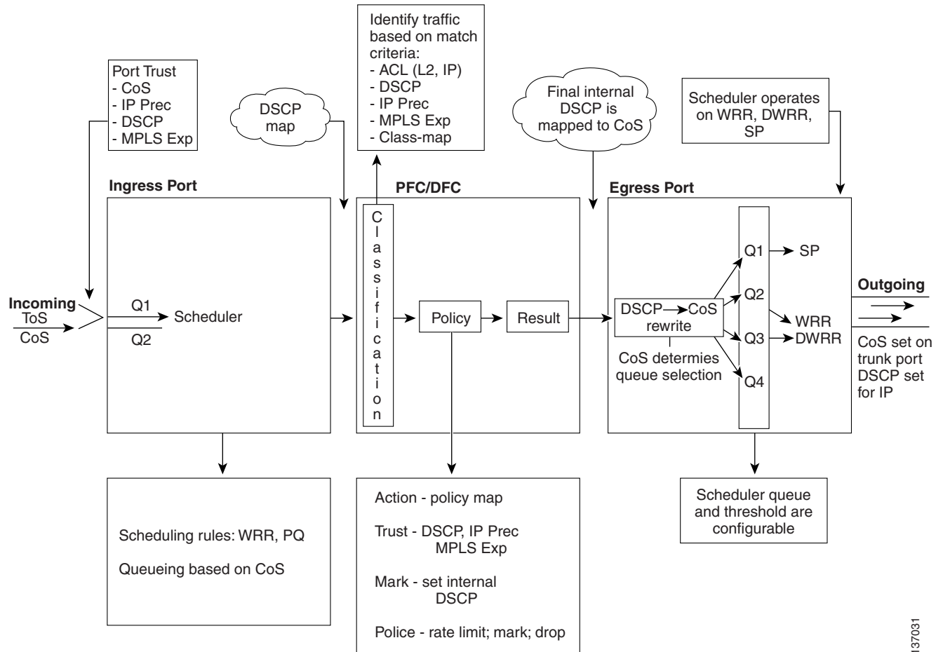
Figure 42-4 PFC QoS Features and Component Overview
