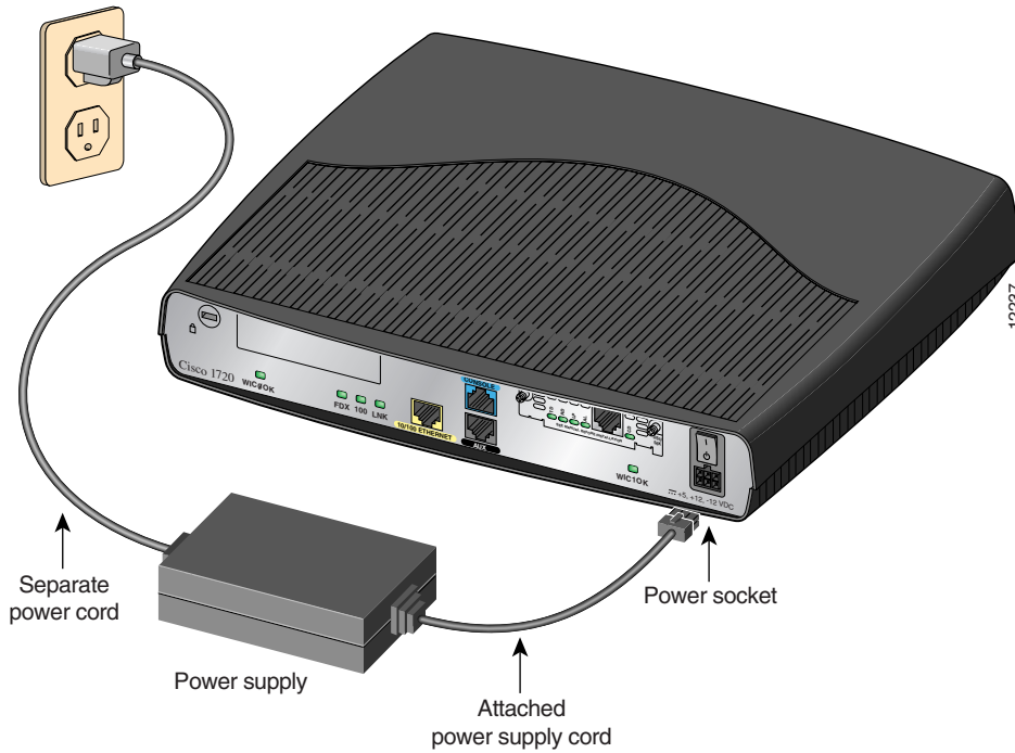
Figure 5 Connecting the Power Supply
