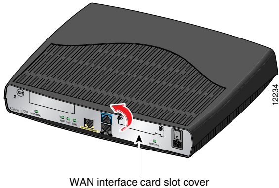
Figure 2 Locating the WAN Interface Card
