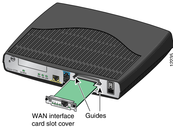
Figure 3 Installing the WAN Interface Card
