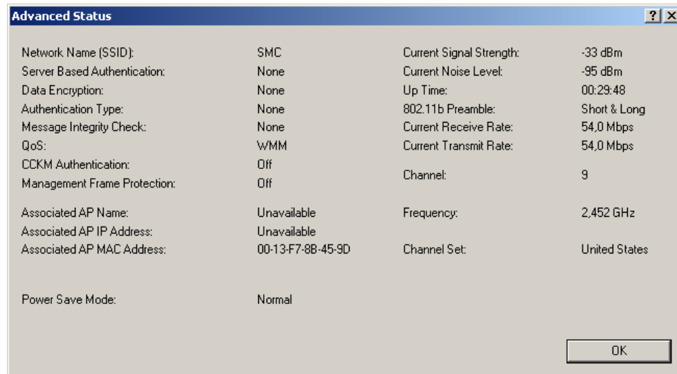
Figure 3-2 Advance Status
