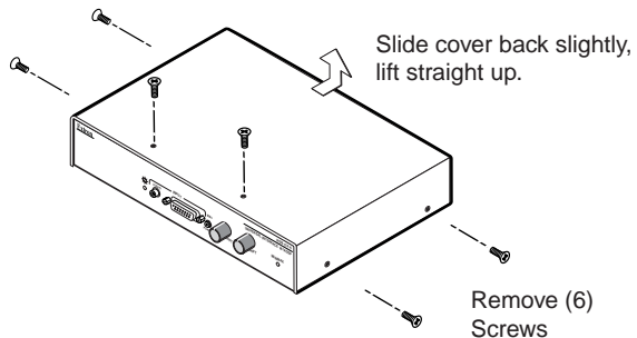
Figure 2-15 — Opening the interface cover
