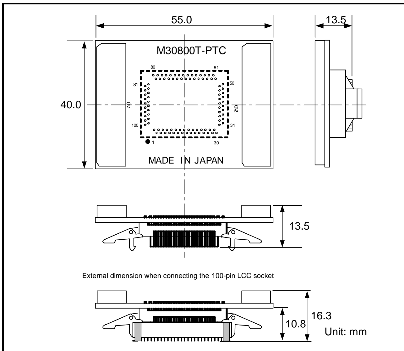
Figure 4.3 External dimensions of the M30800T-PTC
