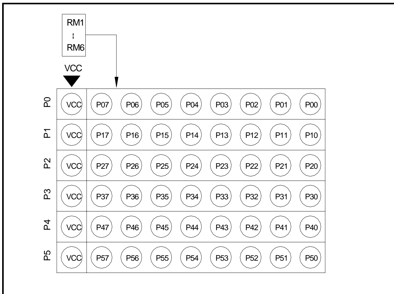
Figure 2.21 Position for mounting network resistors for pullup
