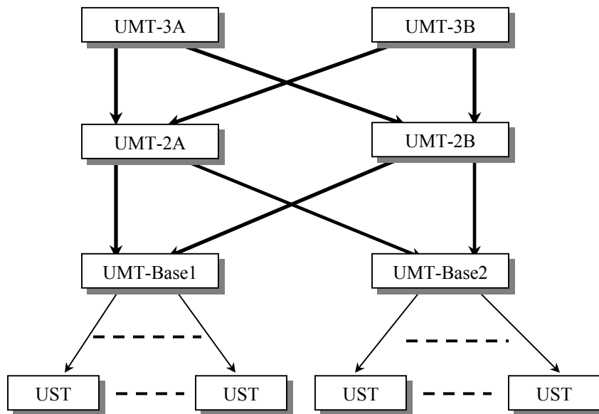
Figure 56 Redundant Configuration
