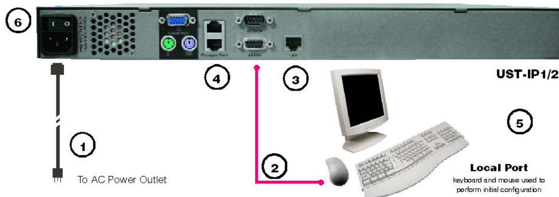
Figure 5 P2-USTIP2 Rear Panel Connections
