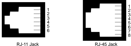
Figure 3. Pin Number Assignments for RJ11 and RJ45 Modular Jacks
