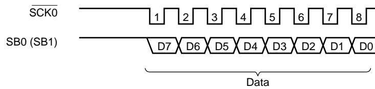
Figure 16-17. Data
