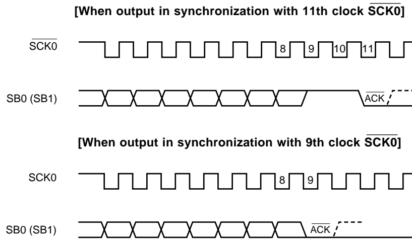
Figure 16-18. Acknowledge Signal
