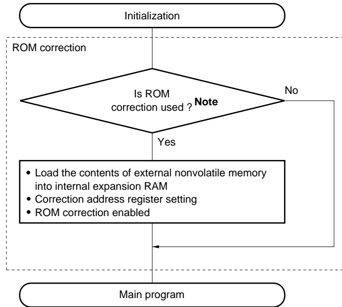
Figure 25-6. Initialization Routine
