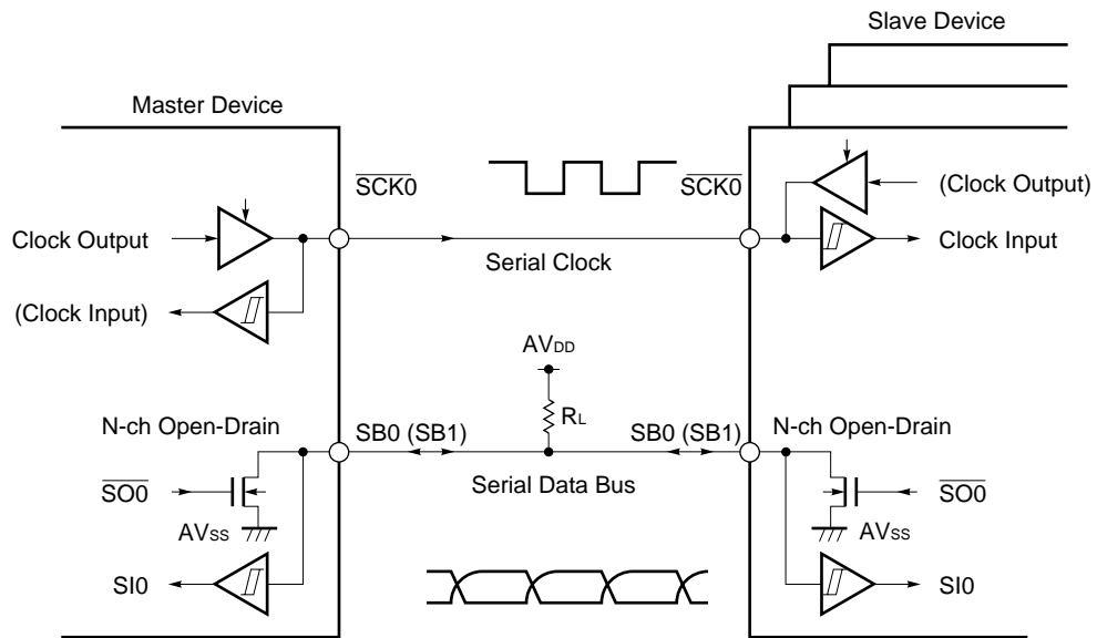
Figure 16-26. Pin Configuration
