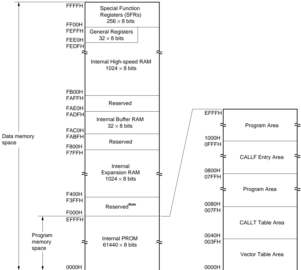
Figure 5-3. Memory Map ( \mu PD78P058F, \mu PD78P058FY)
