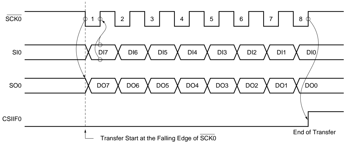
Figure 16-7. 3-Wire Serial I/O Mode Timings
