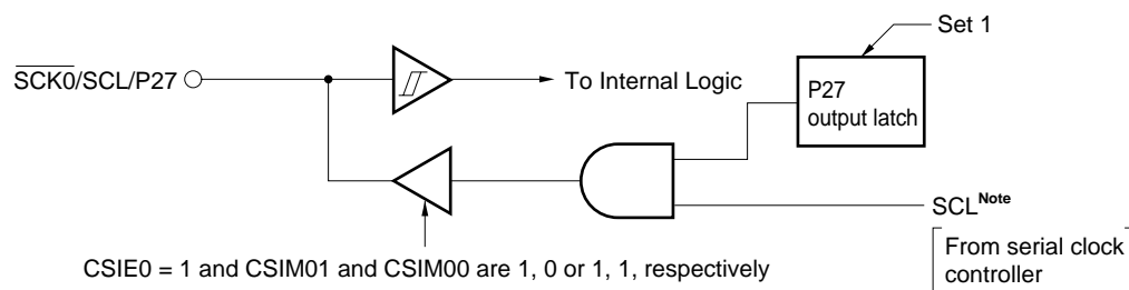
Figure 17-28. \overline{\text{SCK0/SCL/P27}} Pin Configuration
