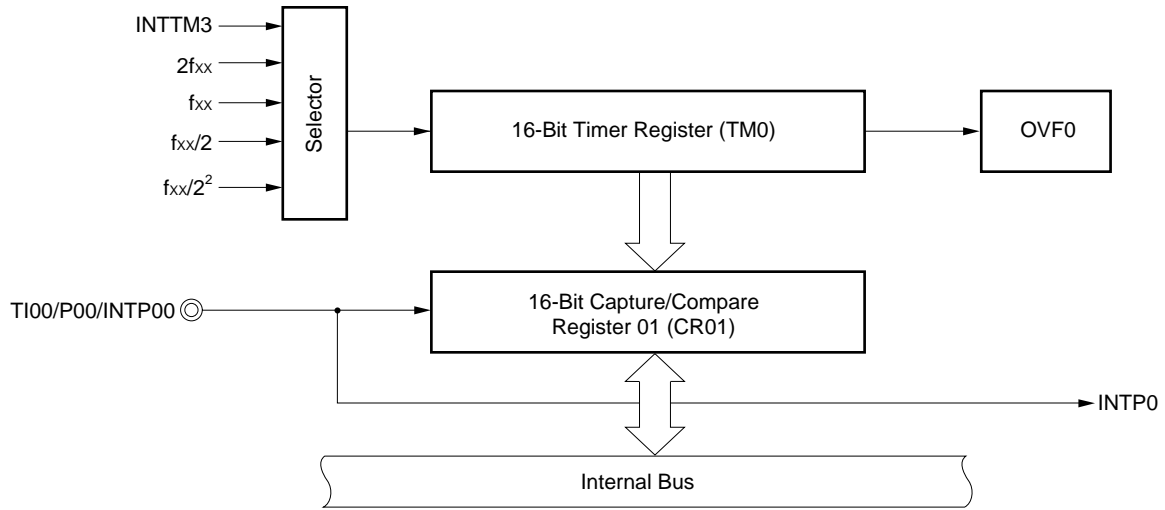
Figure 8-18. Configuration Diagram for Pulse Width Measurement by Free-Running Counter
