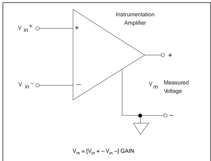
Figure 3-2. DAQCard-1200 Instrumentation Amplifier
