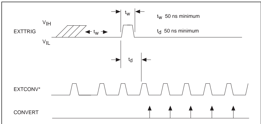
Figure 3-13. Posttrigger DAQ Timing
