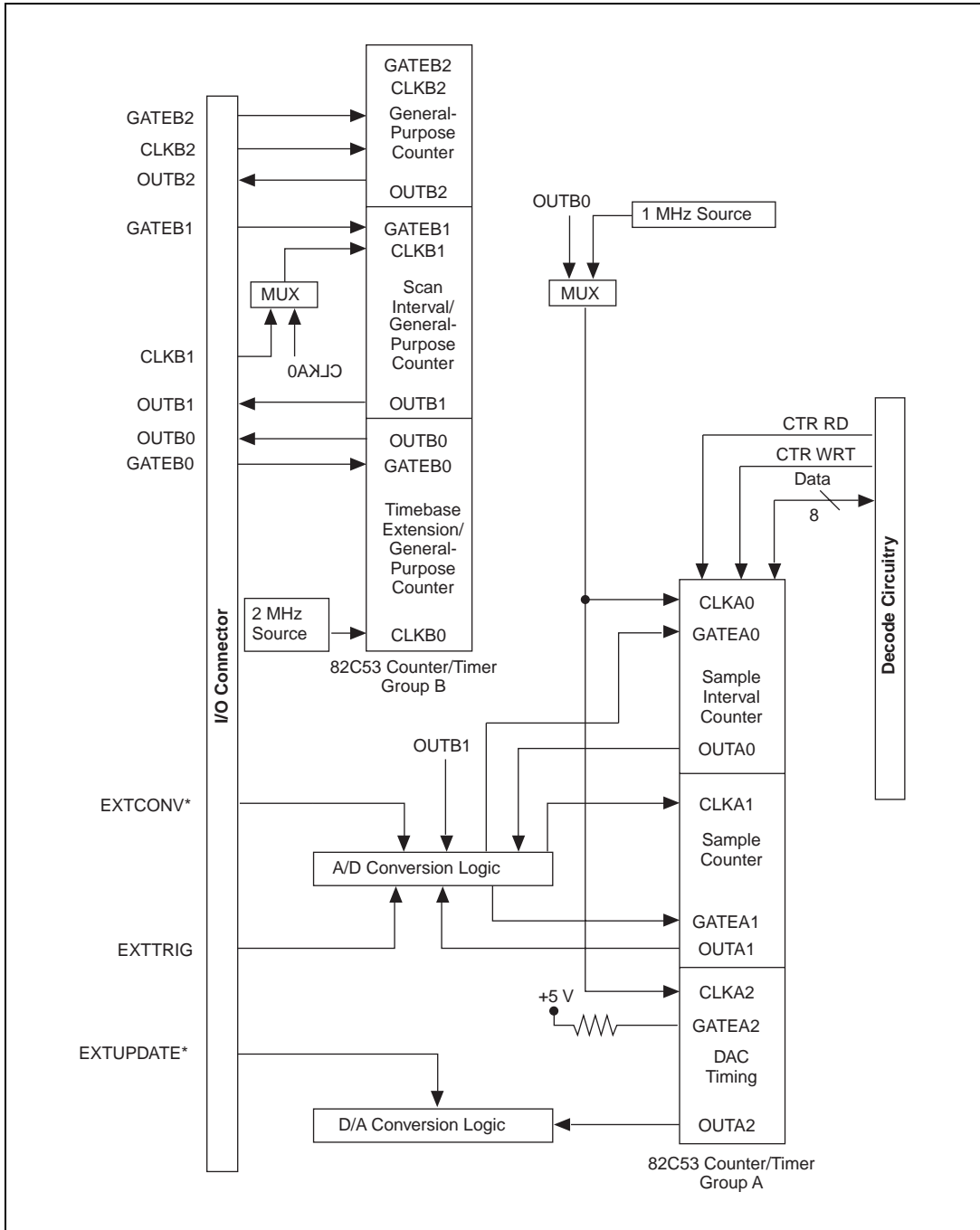
Figure 4-3. Timing Circuitry
