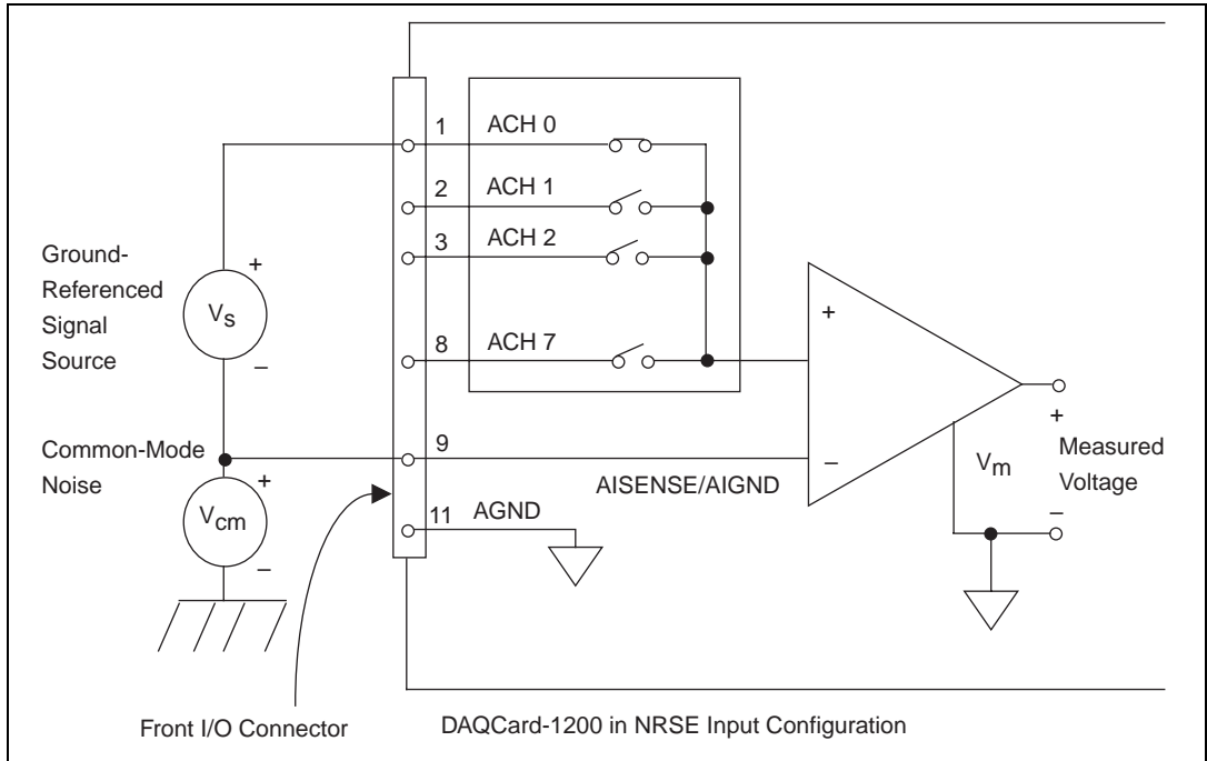
Figure 3-6. Single-Ended Input Connections for Grounded Signal Sources
