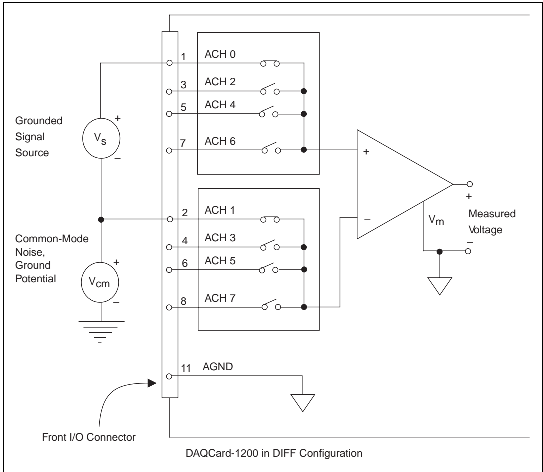
Figure 3-3. Differential Input Connections for Grounded Signal Sources
