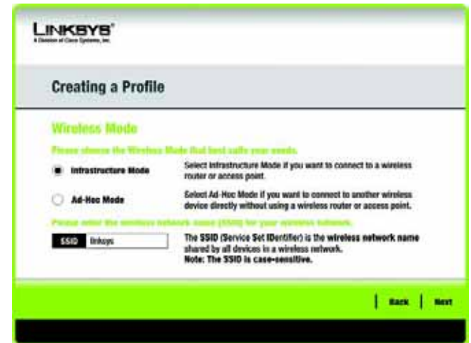
Figure 4-16: Wireless Mode
