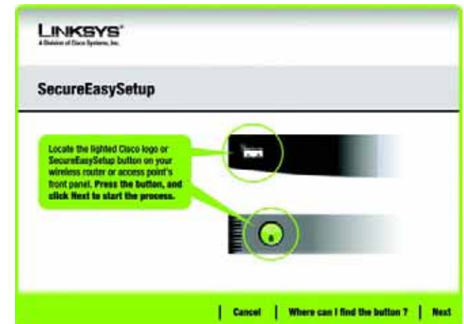
Figure 5-20: SecureEasySetup
