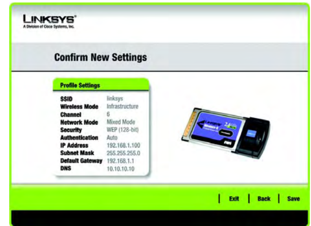
Figure 4-19: Confirm New Settings
