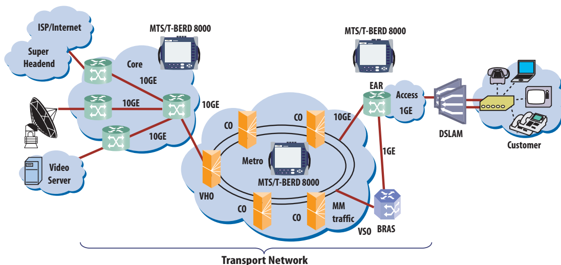
Figure 1 - Network Deployment - Video Services
