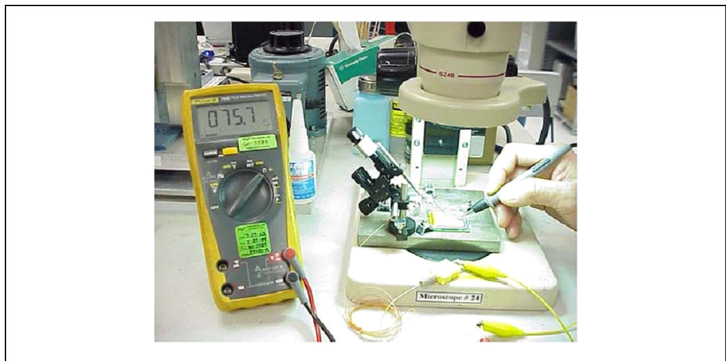
Figure 13. Measuring Resistance between Thermocouple and IHS
