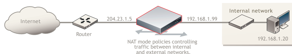
Figure 2: FortiGate unit in NAT mode
