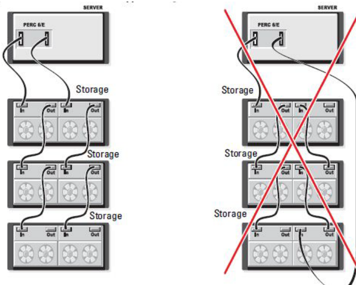
Figure 5. Redundant Path with 3 Enclosures
