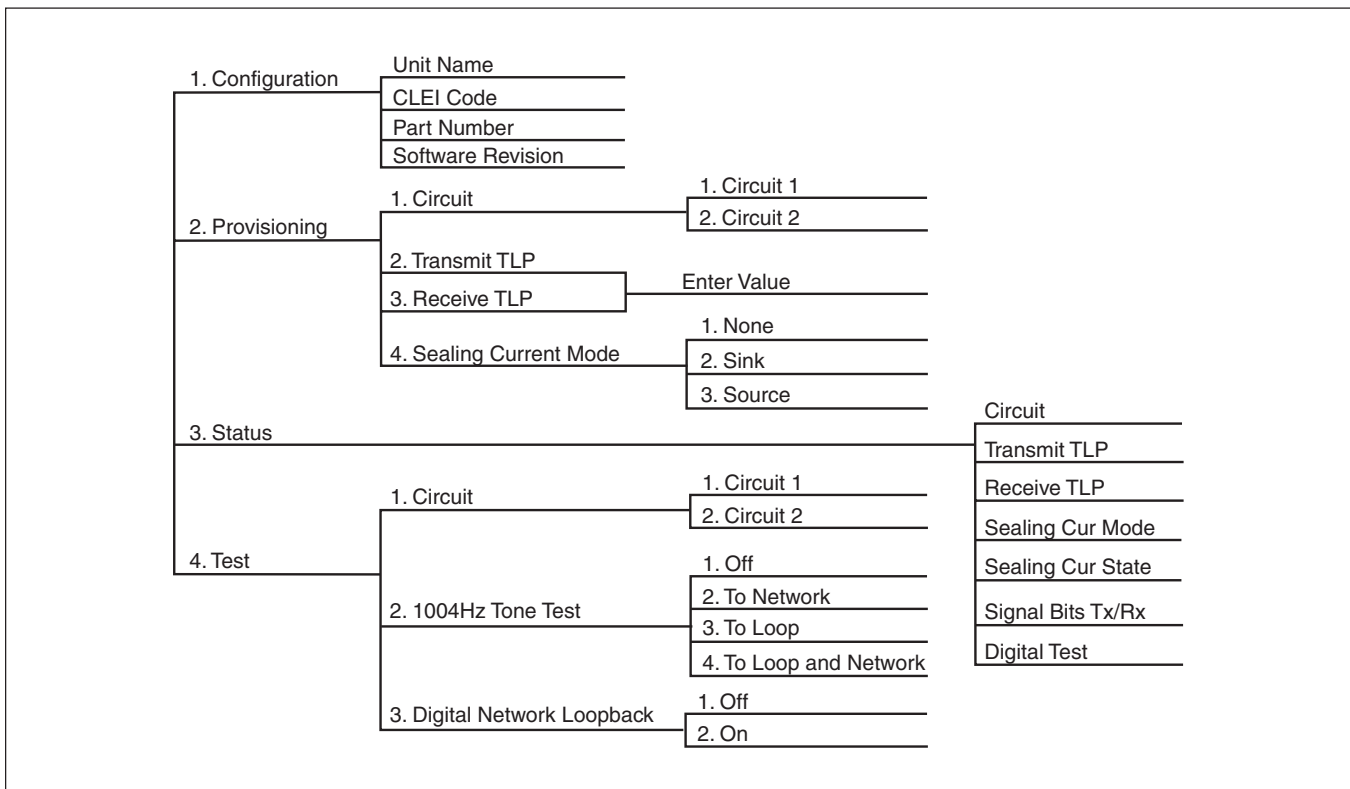
Figure 2. Dual 4-Wire TO Menu Tree
