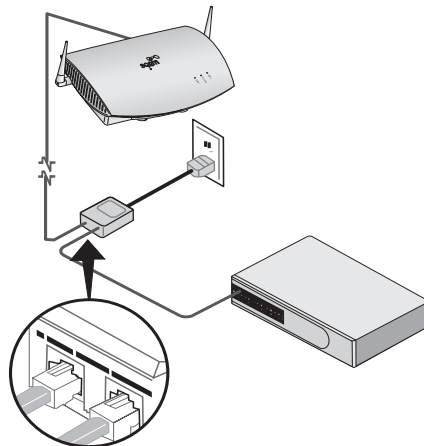
Using an Optional Power-over-Ethernet Injector
