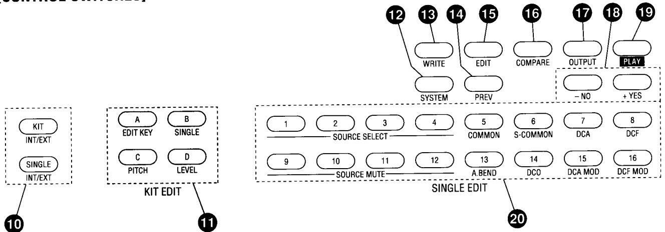
[CONTROL SWITCHES]
