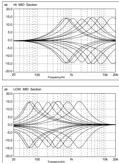
Frequency Response Curves of the Equaliser
