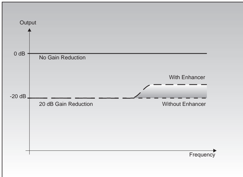
Fig. 3.3: The frequency response with and without dynamic enhancer
