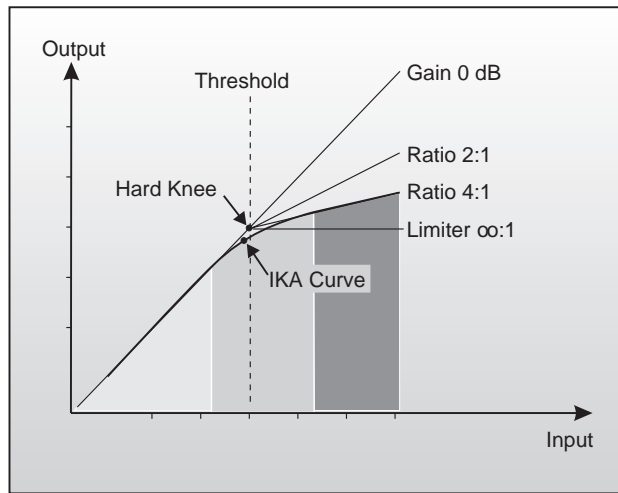
Fig. 3.2: IKA characteristic of the compressor section
