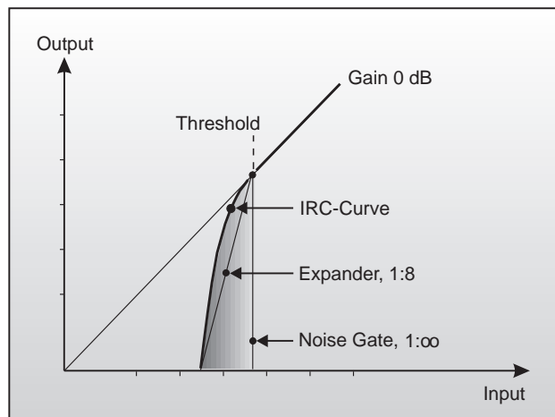
Fig. 3.1: IRC curve characteristic of the Expander
