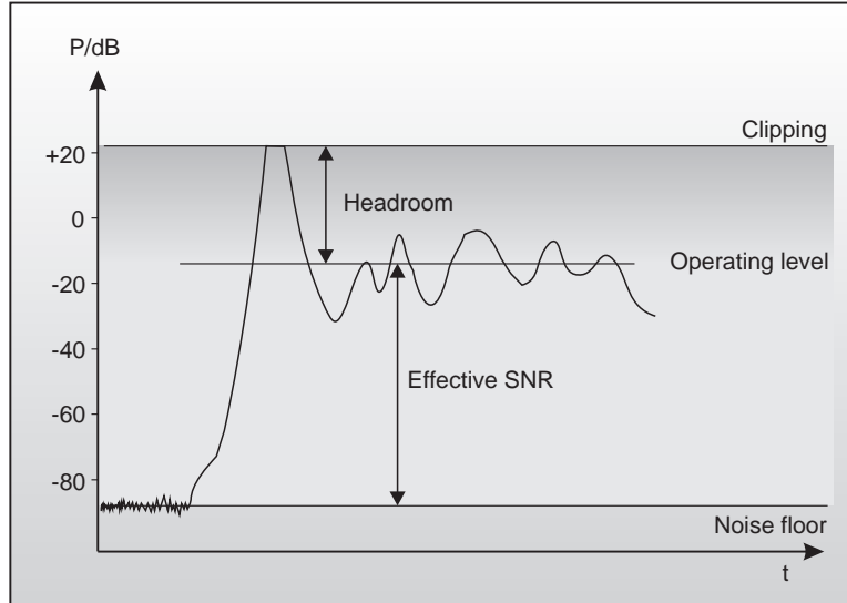
Fig. 6.2: The interactive relationship between the operating level and the headroom
