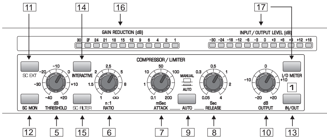
Fig. 2.3: Control elements of the compressor section
