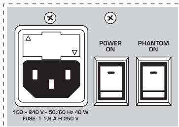
Fig. 2.15: Voltage supply and fuse
