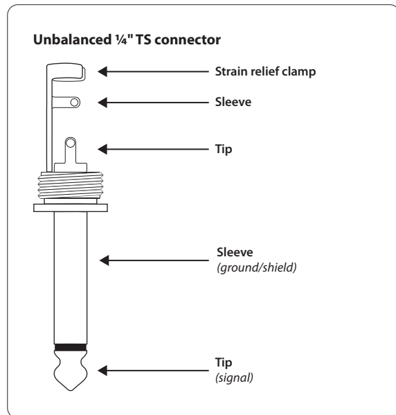
Fig. 4.3: 1/4" TS connector
