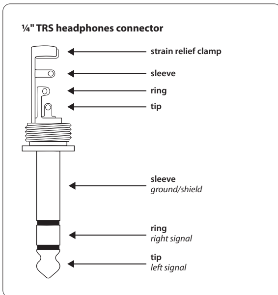
Fig. 4.5: ¼" TRS connector for headphones
