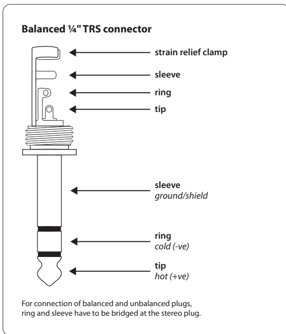
Fig. 4.4: ¼" TRS connector
