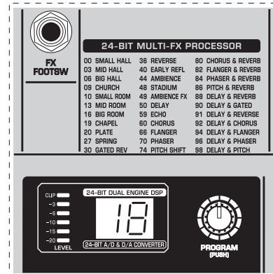
Fig. 3.1: Digital effects module (only 1204FX)
