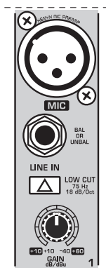
Fig. 2.1: Connectors and controls of mic/line inputs
