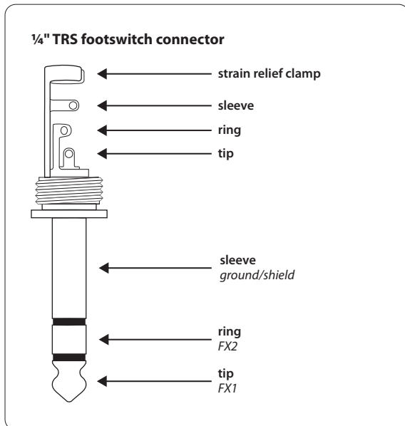
Fig. 4.1: 1/4" TS connector for foot switch
