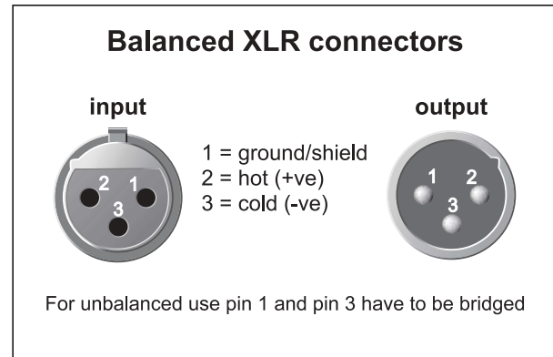
Fig. 3.1: XLR connections
