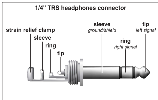
Fig. 3.4: 1/4" TRS headphone connector
