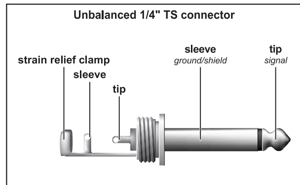
Fig. 3.2: 1/4" TS connector
