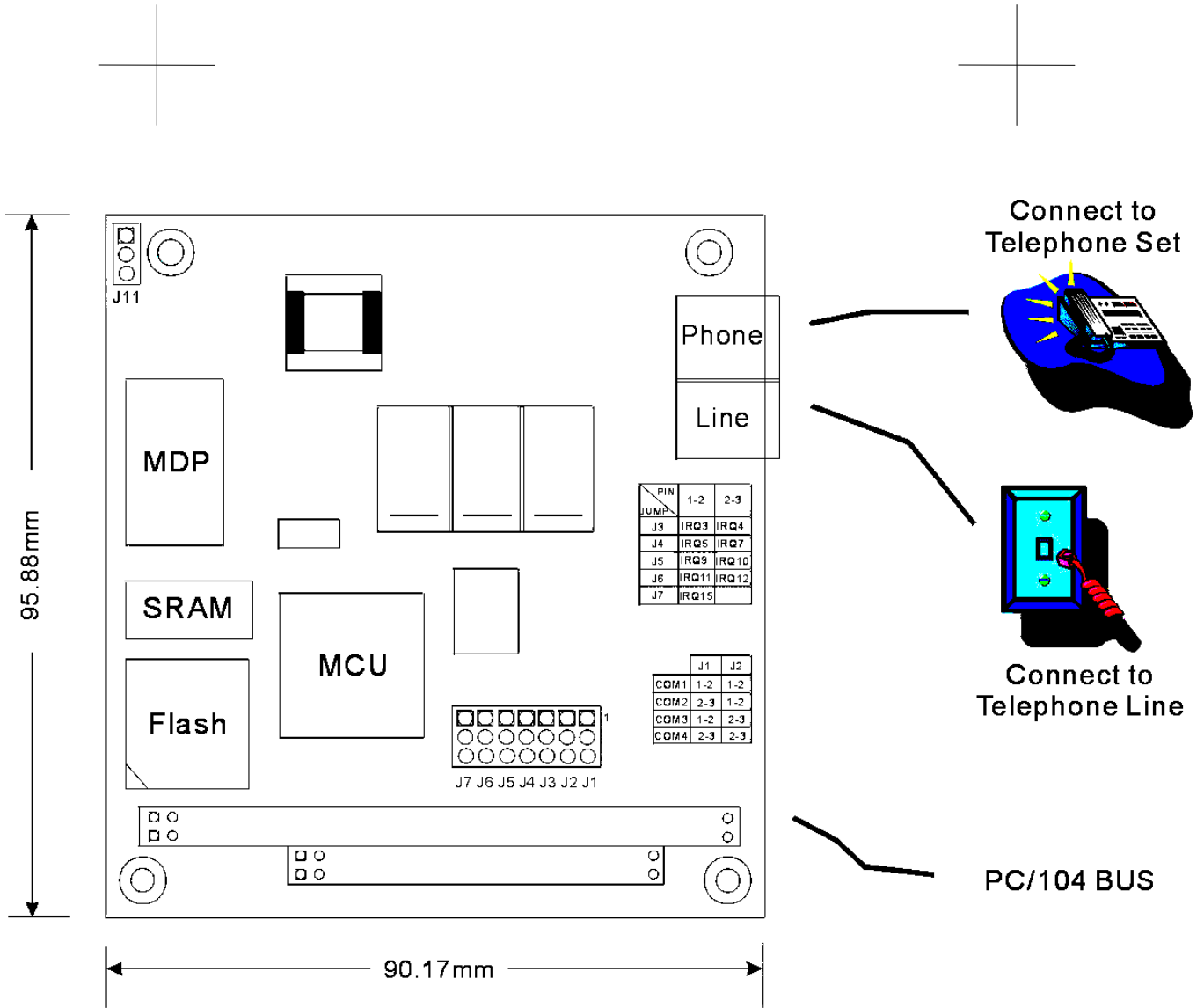
Fig 1-1. PC/104 FaxModem Card
