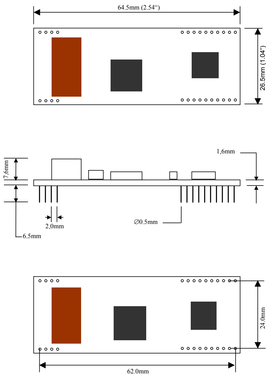
Figure 4-1. AL5068S Socket Modem Physical Dimensions
